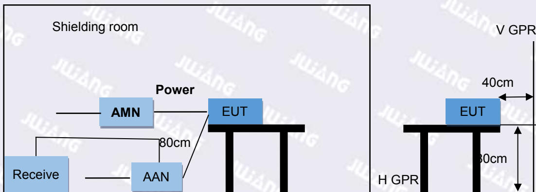
Figure 5-6 Test set-up of conducted disturbance for wired network ports
